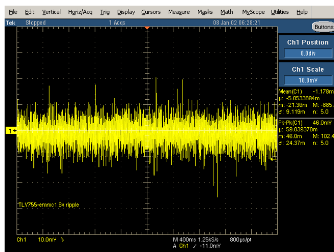
Fig. 4: Main_eMMC_VDDQ_ripple
